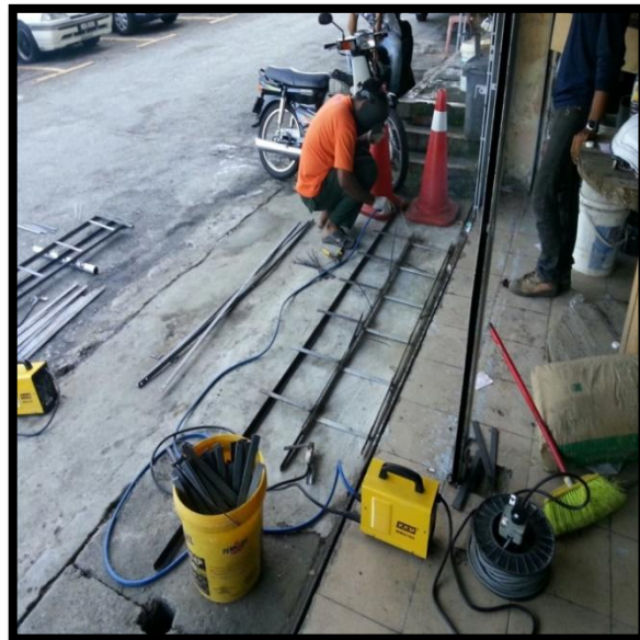
FABRICATE CABLE LADDER
