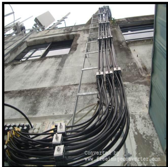
GABS HUAWEI FIBER INSTALLTION
