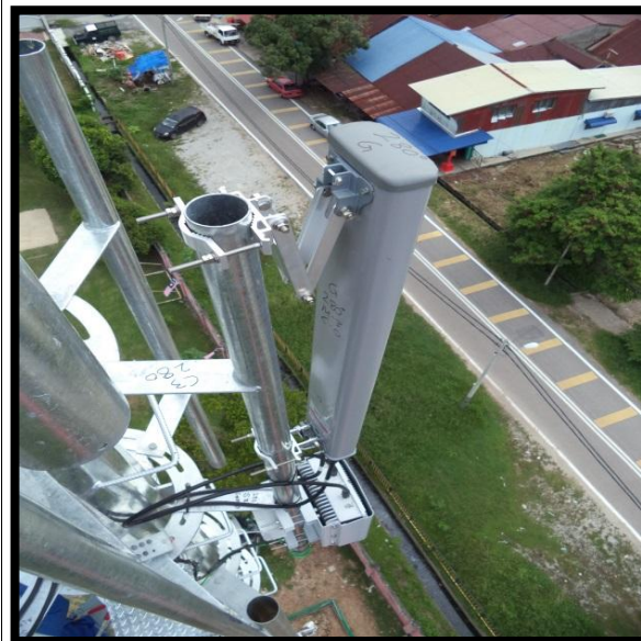
ANTENNA INSTALLATION
