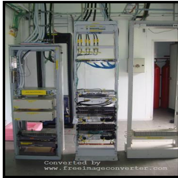
LINK HUAWEI 19 INCH RACK INSTALLTION
